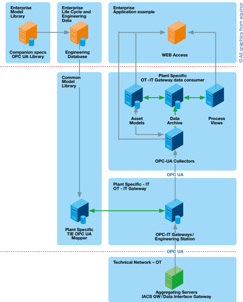
Figure 3: OPC UA Aggregation Architecture
