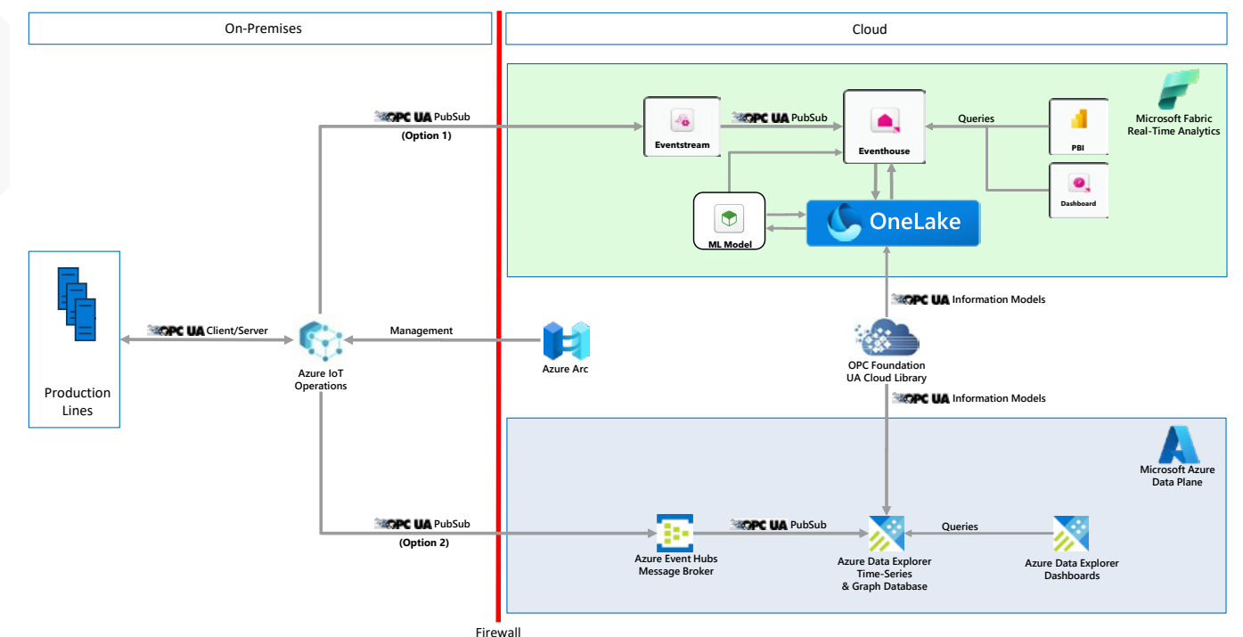
Azure Industrial IoT Reference Architecture
