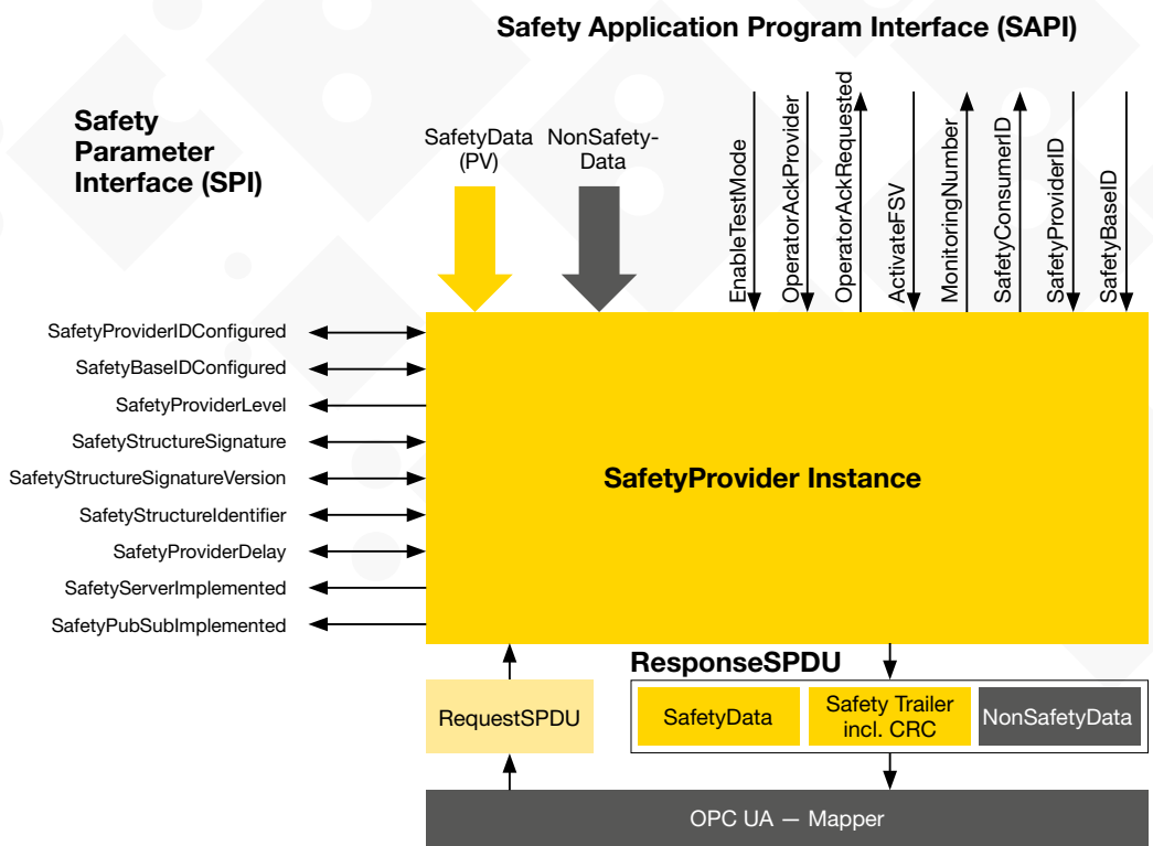
Figure 4: Interfaces of the SafetyProvider: SAPI, SPI and SPDUs.
