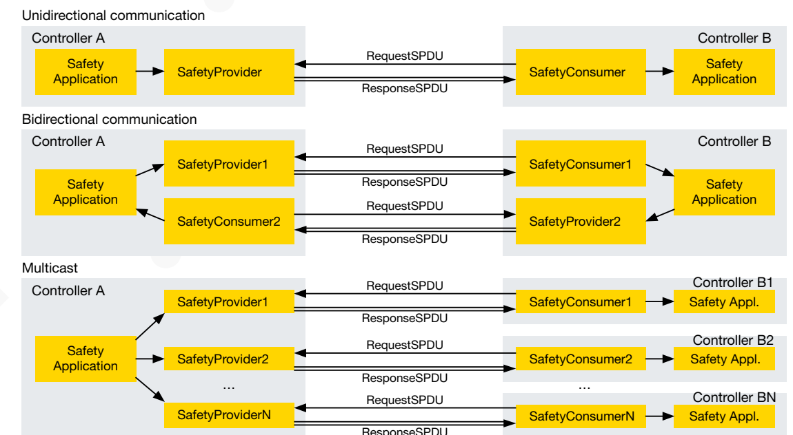
Figure 2: Communication relationships: Unidirectional and bidirectional unicast, as well as multicast.
