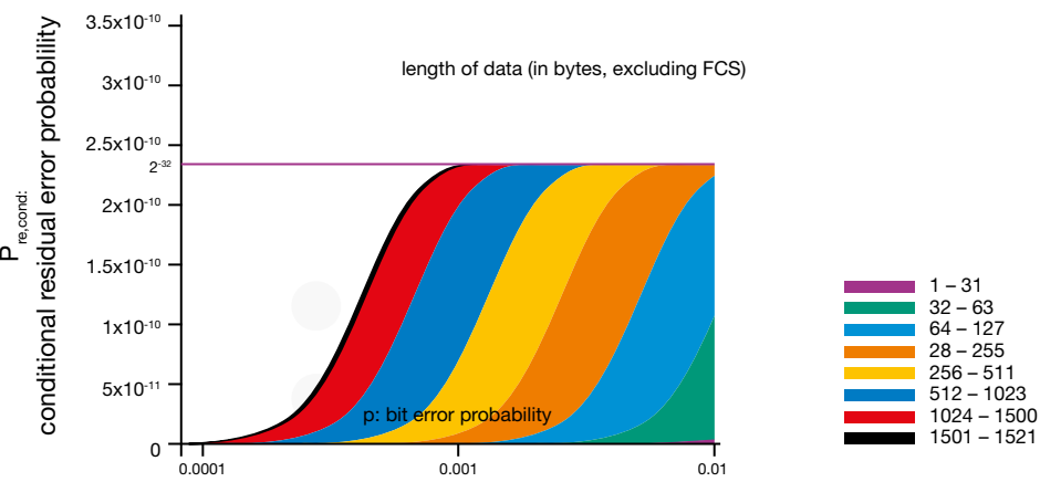
Figure 12: Conditional residual error probability of the CRC procedure used in OPC UA for message lengths of 1-1,521 bytes and all relevant bit error probabilities p.
