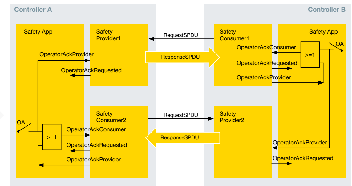
Figure 9: Bidirectional communication where operator acknowledgement is possible on both sides.
