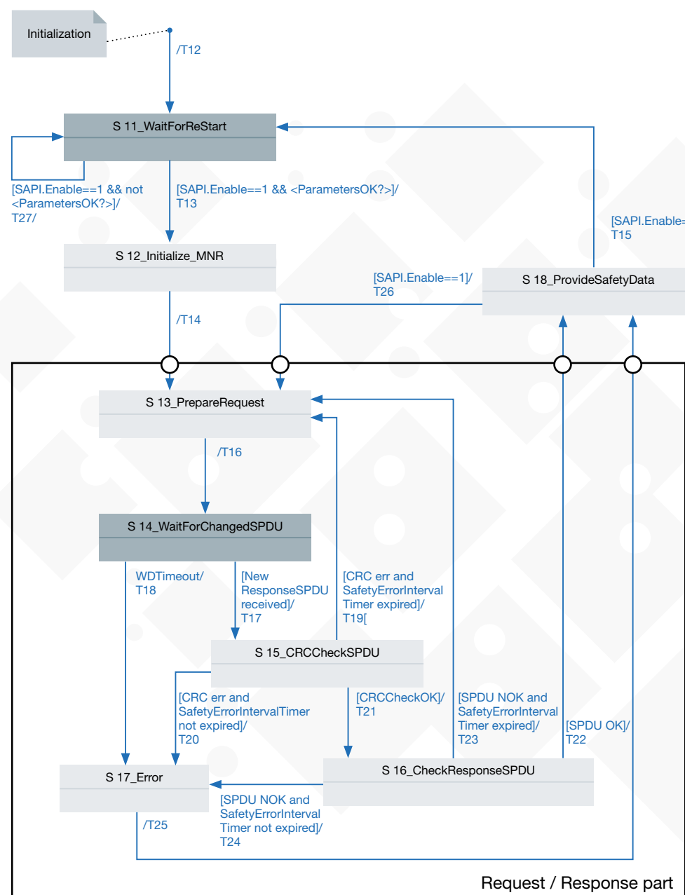
Figure 8: State diagram of the SafetyConsumer.
