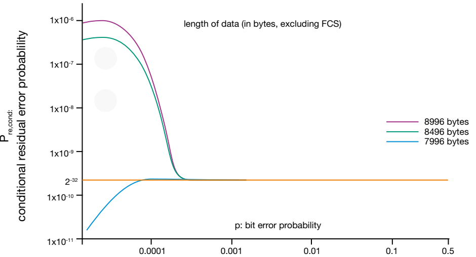
Figure 13: Counter-example: selected message lengths where the conditional residual error probability is much larger than 2^{-32} .
