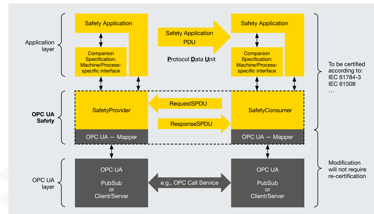
Figure 3: Overview of the OPC UA Safety Architecture
