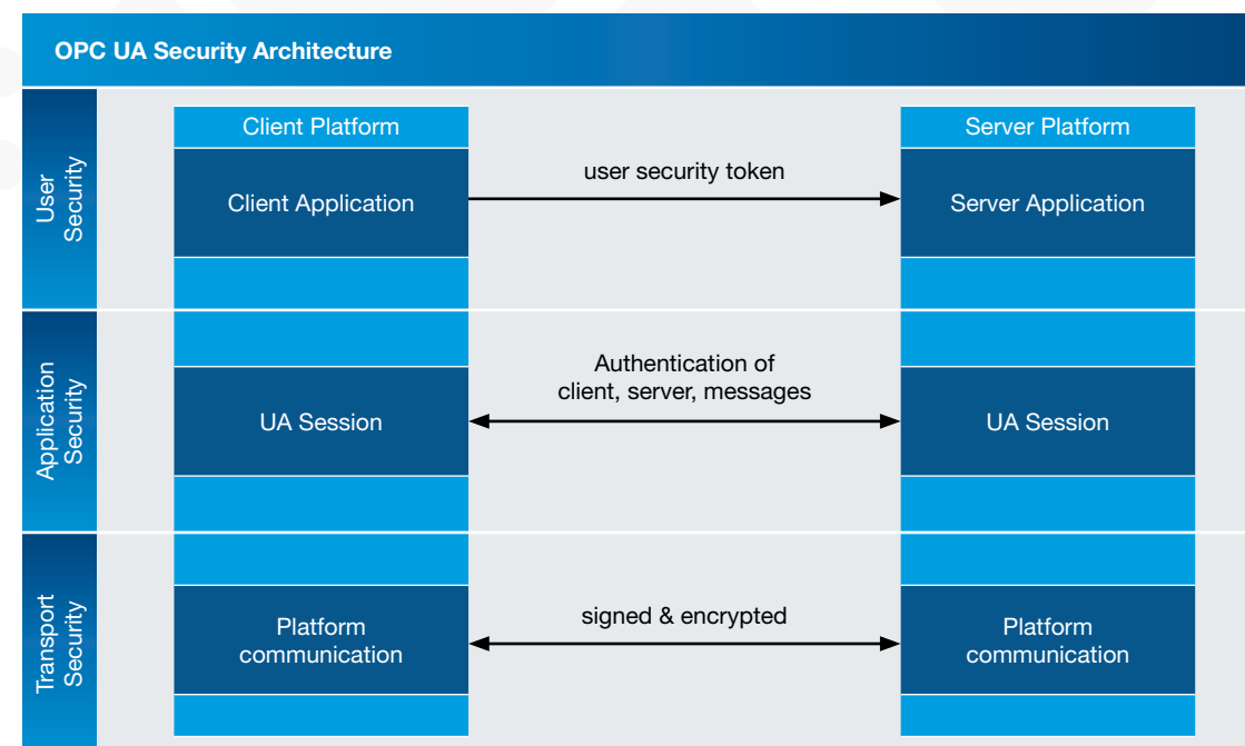
Figure 4: Scalable Security Concept
