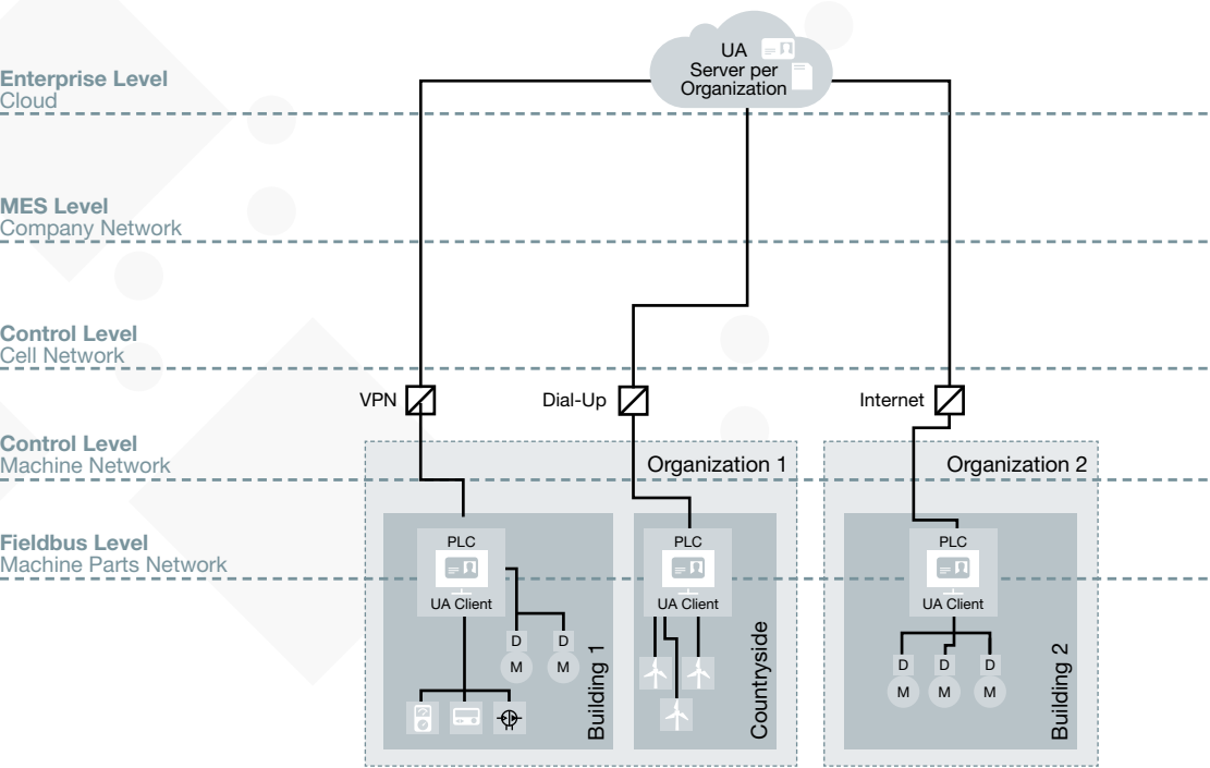
Figure 8: Secure Communication of PLCs with a Cloud for Condition Monitoring of Energy Data
