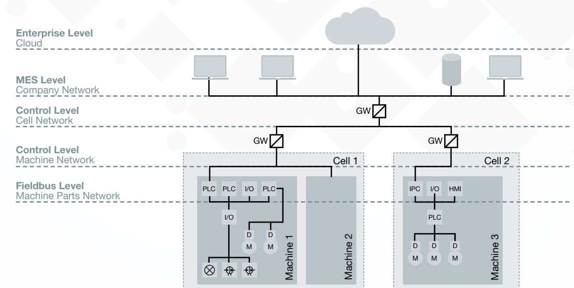
Figure 1: Connected Factory
