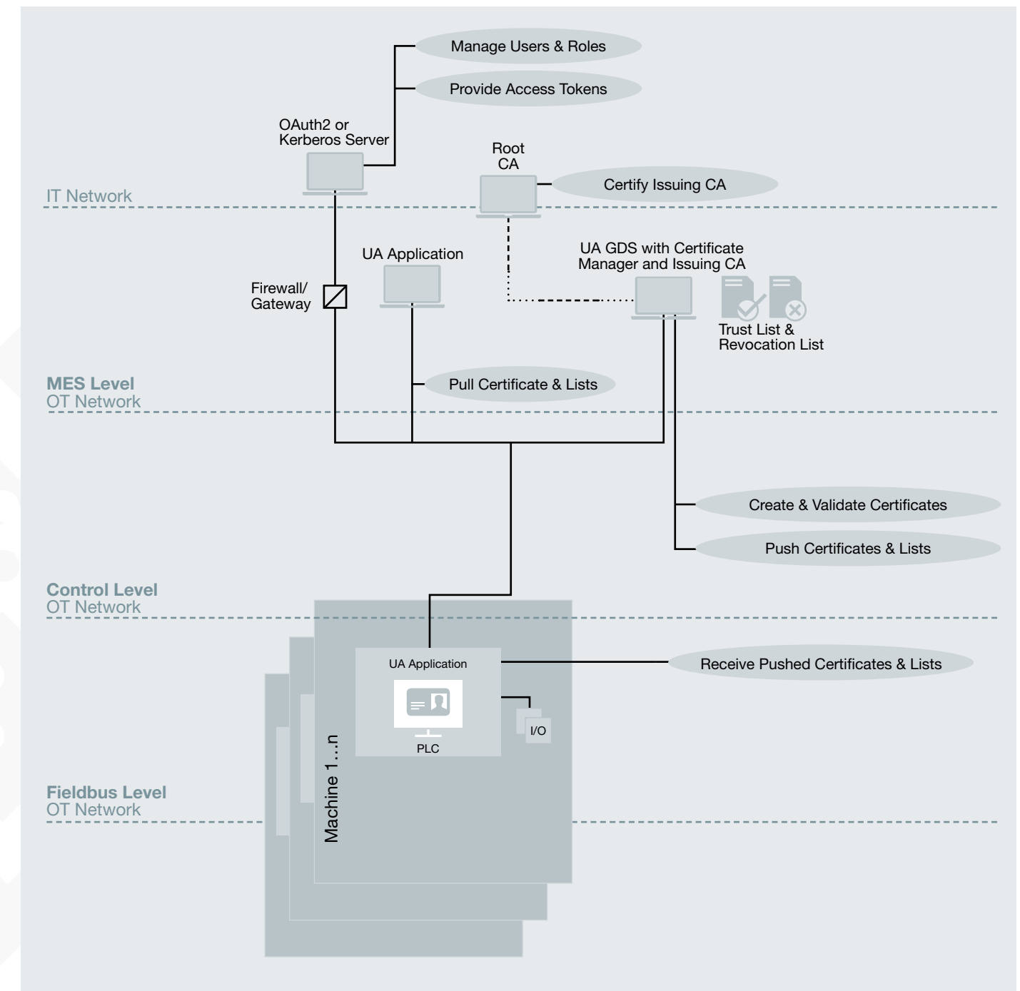
Figure 5: Connected Factory with new UA Features and Use Cases
