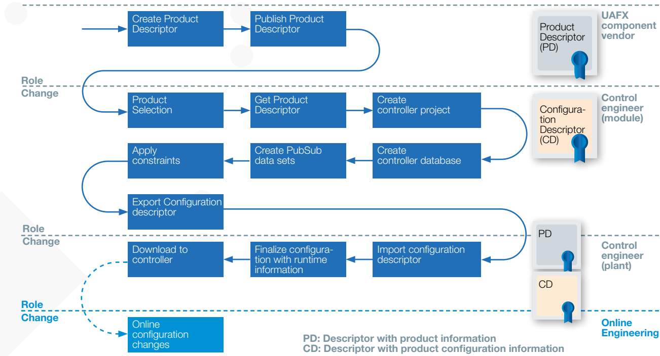
Figure 15: Overview of the workflow steps for offline engineering descriptor(s) usage
