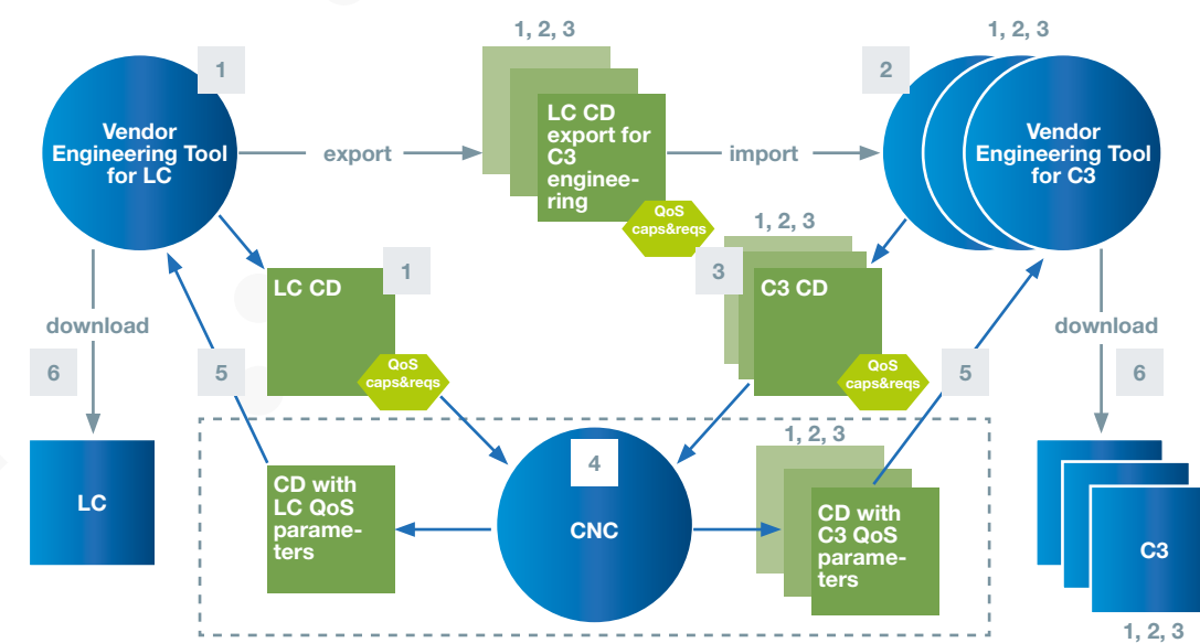
Figure 17: Example: A system with a Line Controller configuring 3 subordinate controllers with TSN
