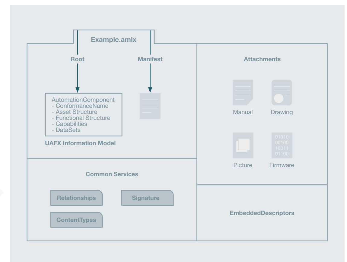
Figure 13: The Product Descriptor
