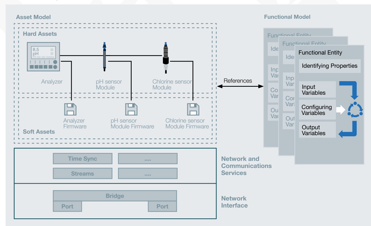
Figure 8: UAFX Automation Component Model
