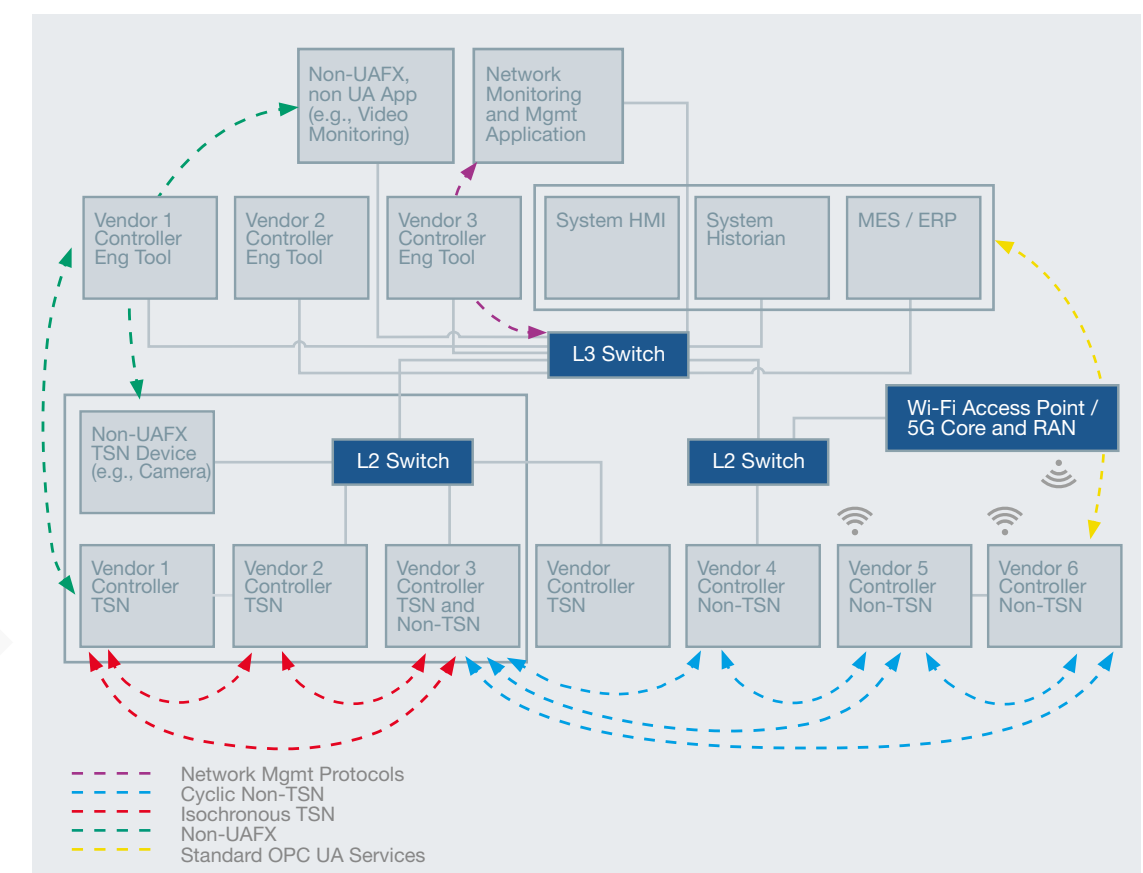
Figure 3: Controller-to-Controller supported network architecture
