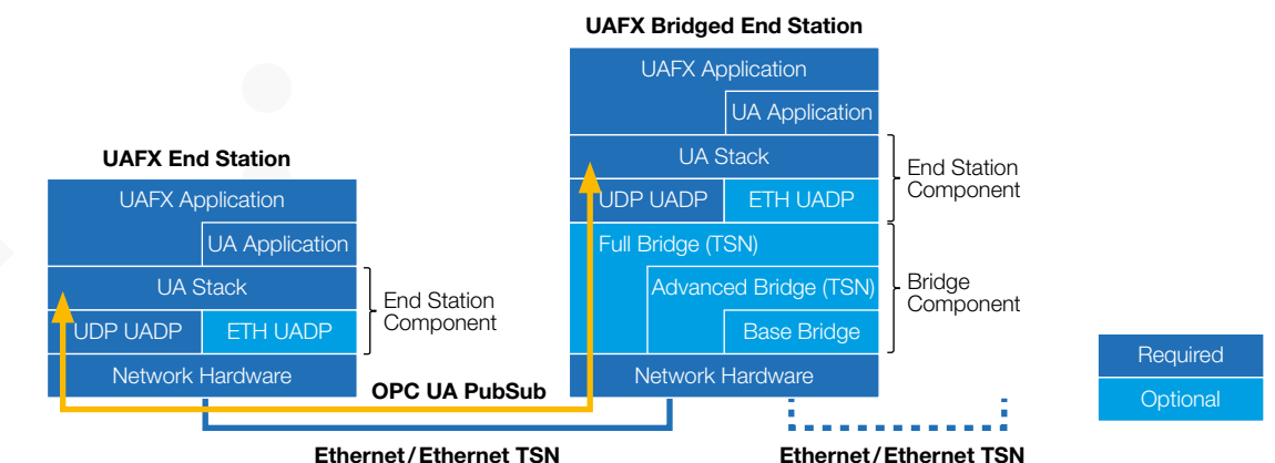
Figure 22: UAFX Transport Architecture
