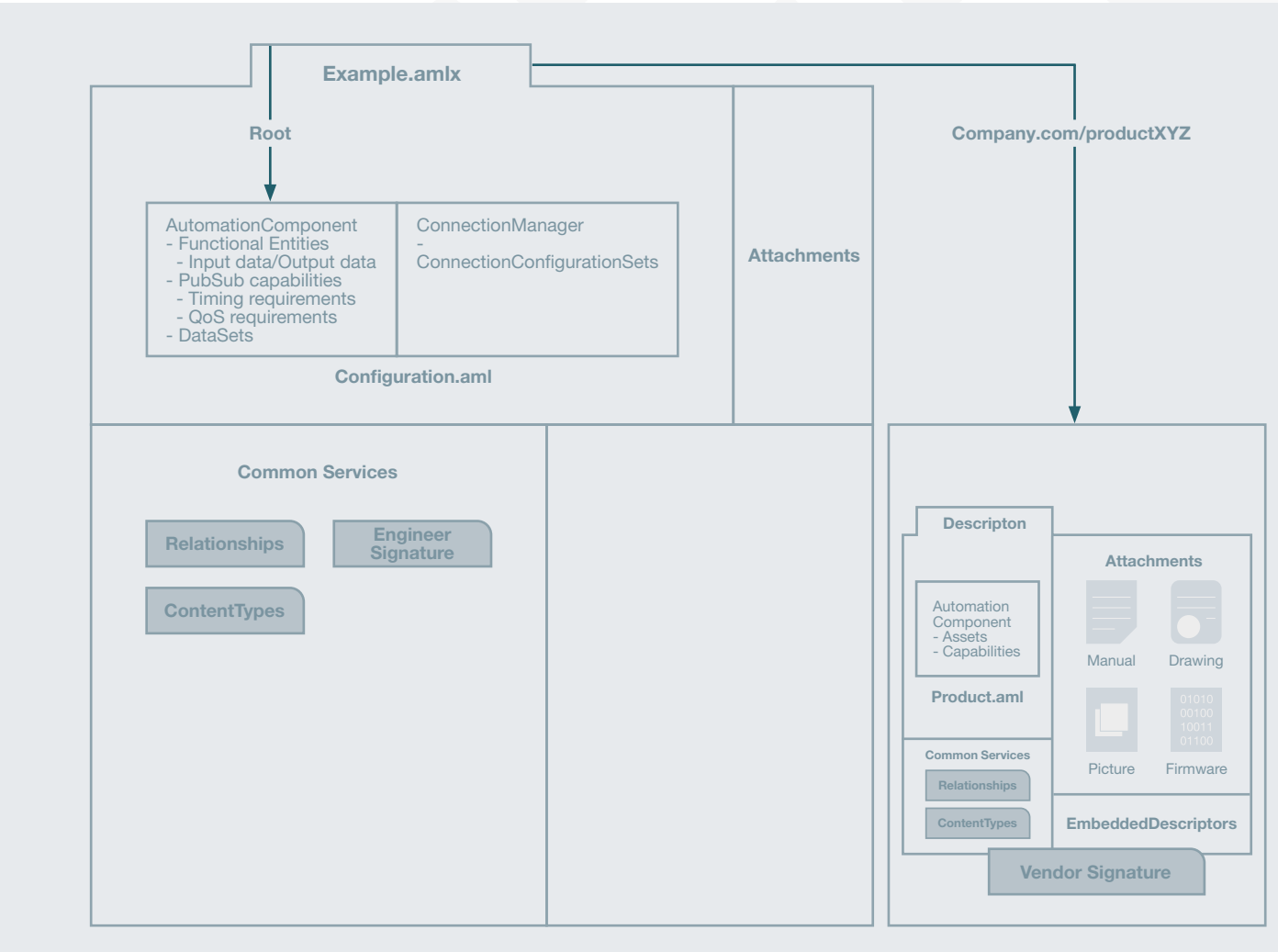
Figure 14: The Configuration Descriptor referencing a Product Descriptor
