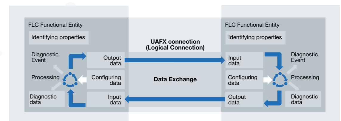
Figure 9: UAFX connections between Functional Entities
